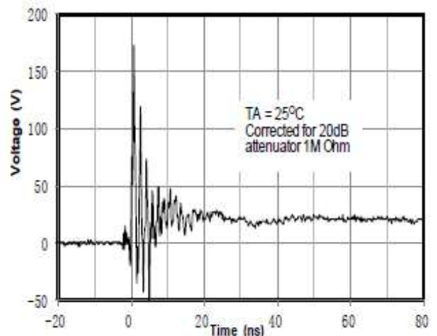
Fig. 6 ESD Clamping Voltage 8kV Contact per IEC61000-4-2
